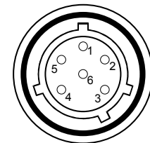
Connector Pin Detail
